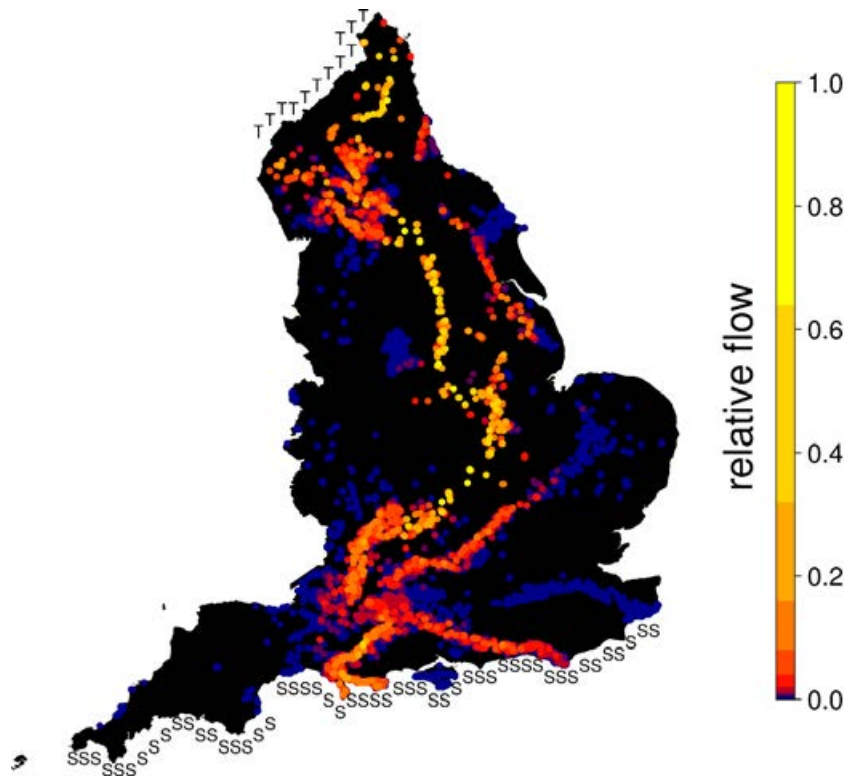
Flow output from Condatis for Lowland Chalk Grassland Habitat using a 4 km dispersal distance with the source defined as the south coast of England (S) and the destination the border between England and Scotland (T), using only priority habitat data for England (Source: Alison et al. 2018). © Natural England 2019. Map produced using Condatis (Wallis, D.W. & Hodgson, J.A. (2018) Condatis 0.6.0. http://wordpress.condatis.org.uk/ ). Contains public sector information licensed under the Open Government Licence v3.0
